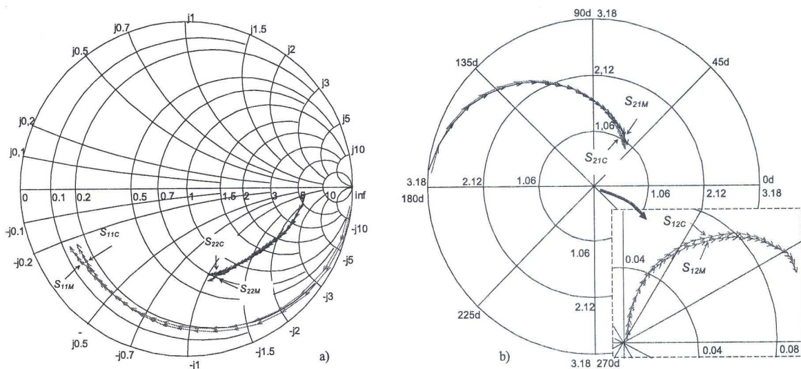
Fig. 3. Measured and simulated S-parameters of MESFET shown in a) Smith chart, b) polar chart. Frequency points are marked in the range 500 MHz – 25.5 GHz with the step of 1 GHz by arrows.
